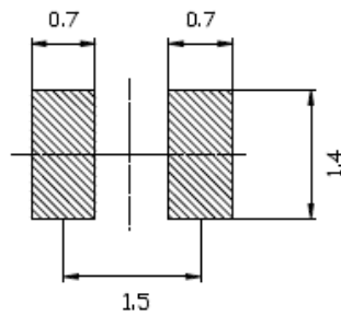
LAND PATTERN(REFERENCE)
